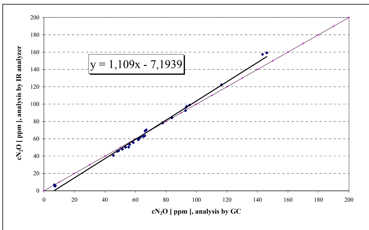
Figure 2 The comparison of the IR and GC analyses of nitrous oxide
