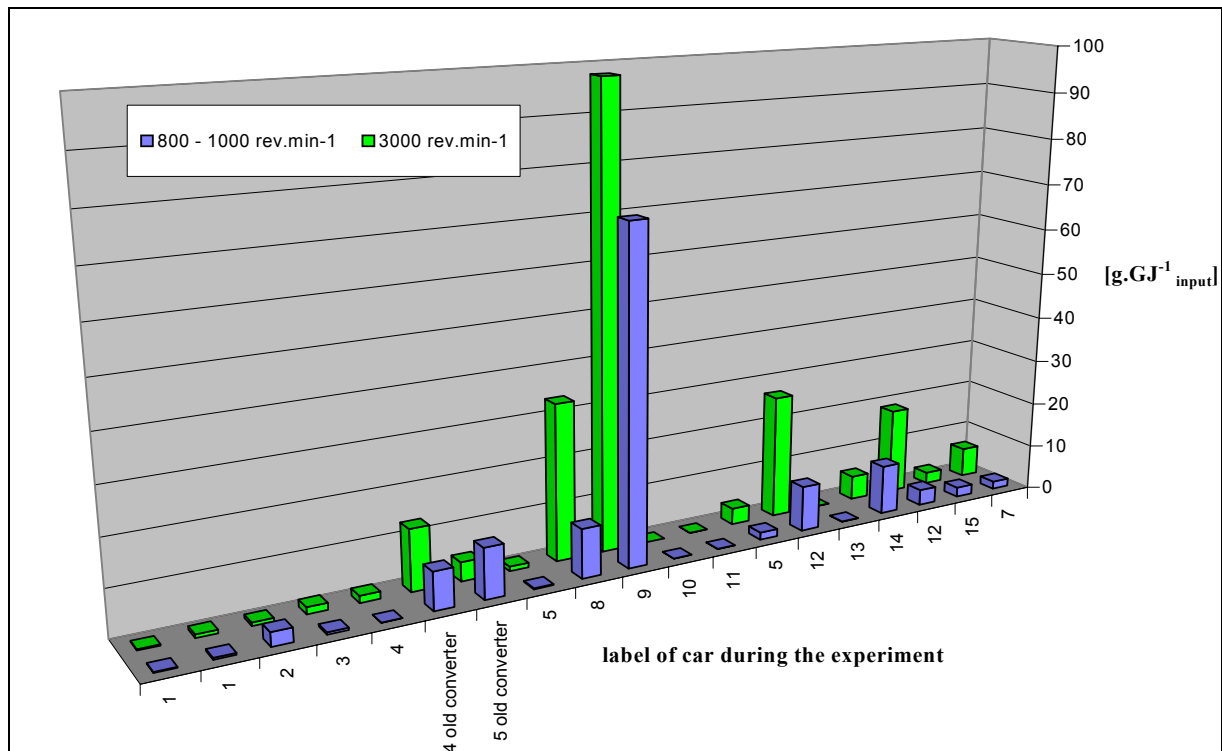
Figure 3 The N 2 O emission factors of the mobile sources in the dependence on their type and output
